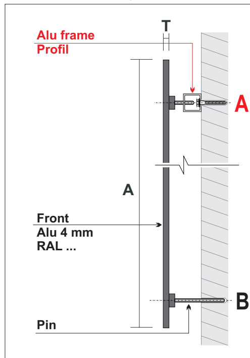
Alu letter mounting with pin
