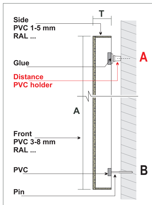
PVC letter mounting with pin
