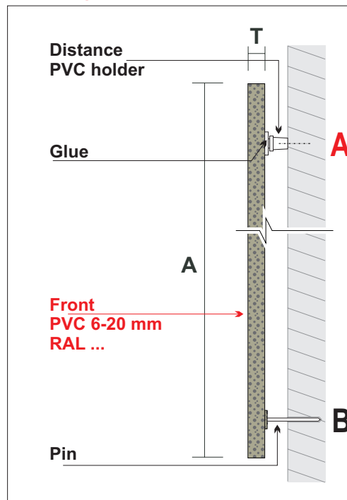
PVC letter mounting with pin
