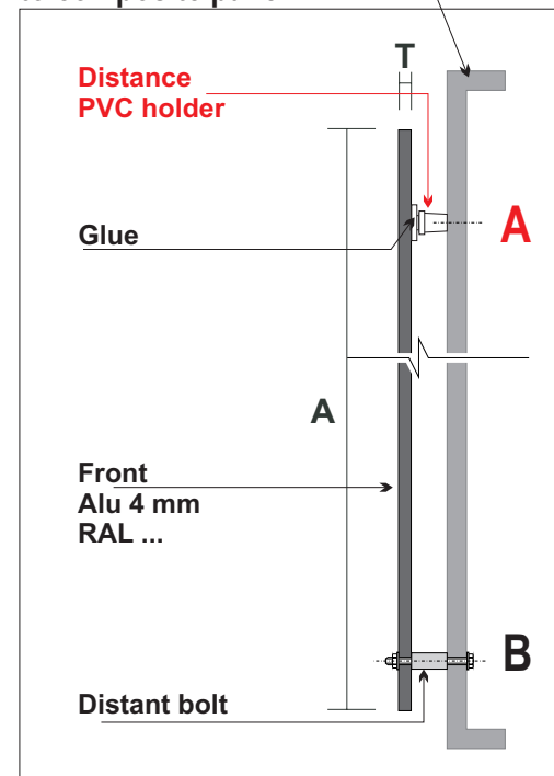
mounting with distant bolt
