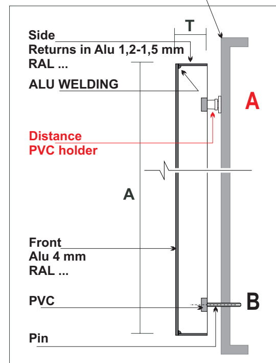
mounting with pin
