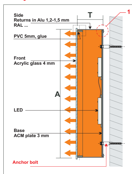
mounting with anchor bolt
