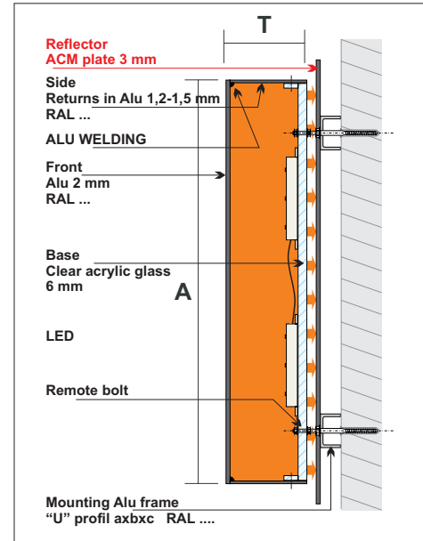
Letter with reflector
