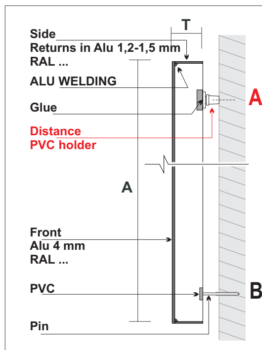
mounting with pin
