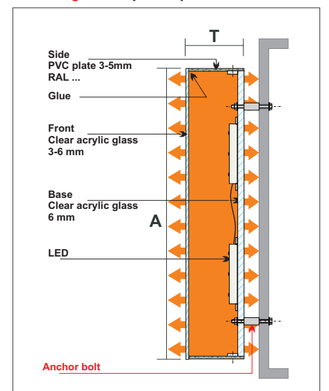
Mounting with anchor bolt
