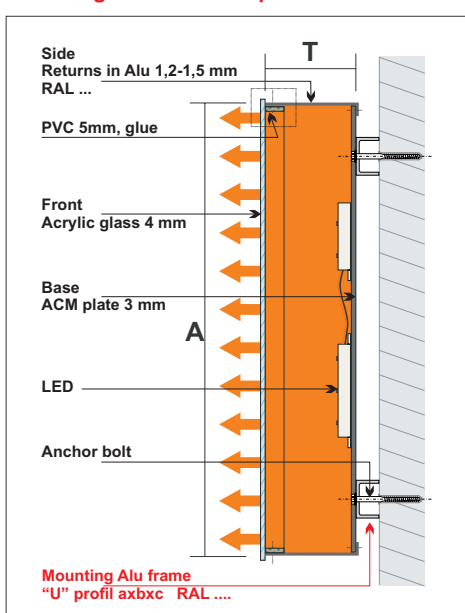
Mounting Alu frame "U" profil
